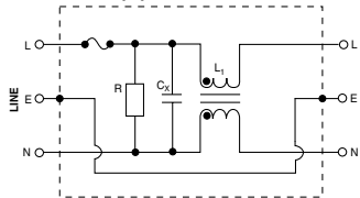
66/67-BFF(S)-XXX-1-X Filter
