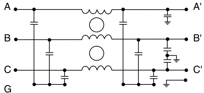
Circuit 2
