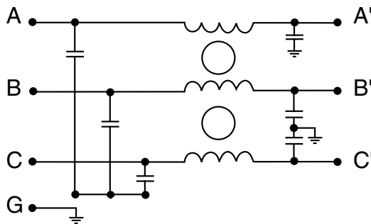
Circuit 1
